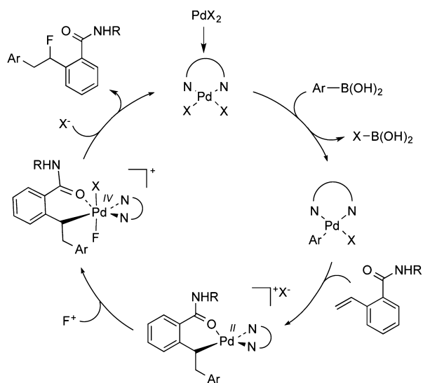
Scheme 4. Proposed Mechanism for the Directed Fluoroarylation of Styrene
